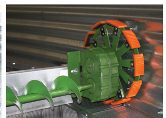
The sweep auger can also be delivered with extra reduced speed on the drive wheel, ratio 16:1 ▼
